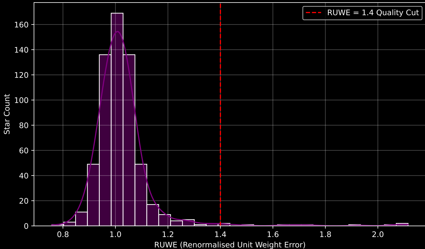
GAPOGEE DR17 Field [020+06] RUWE Distribution (n= 602)
