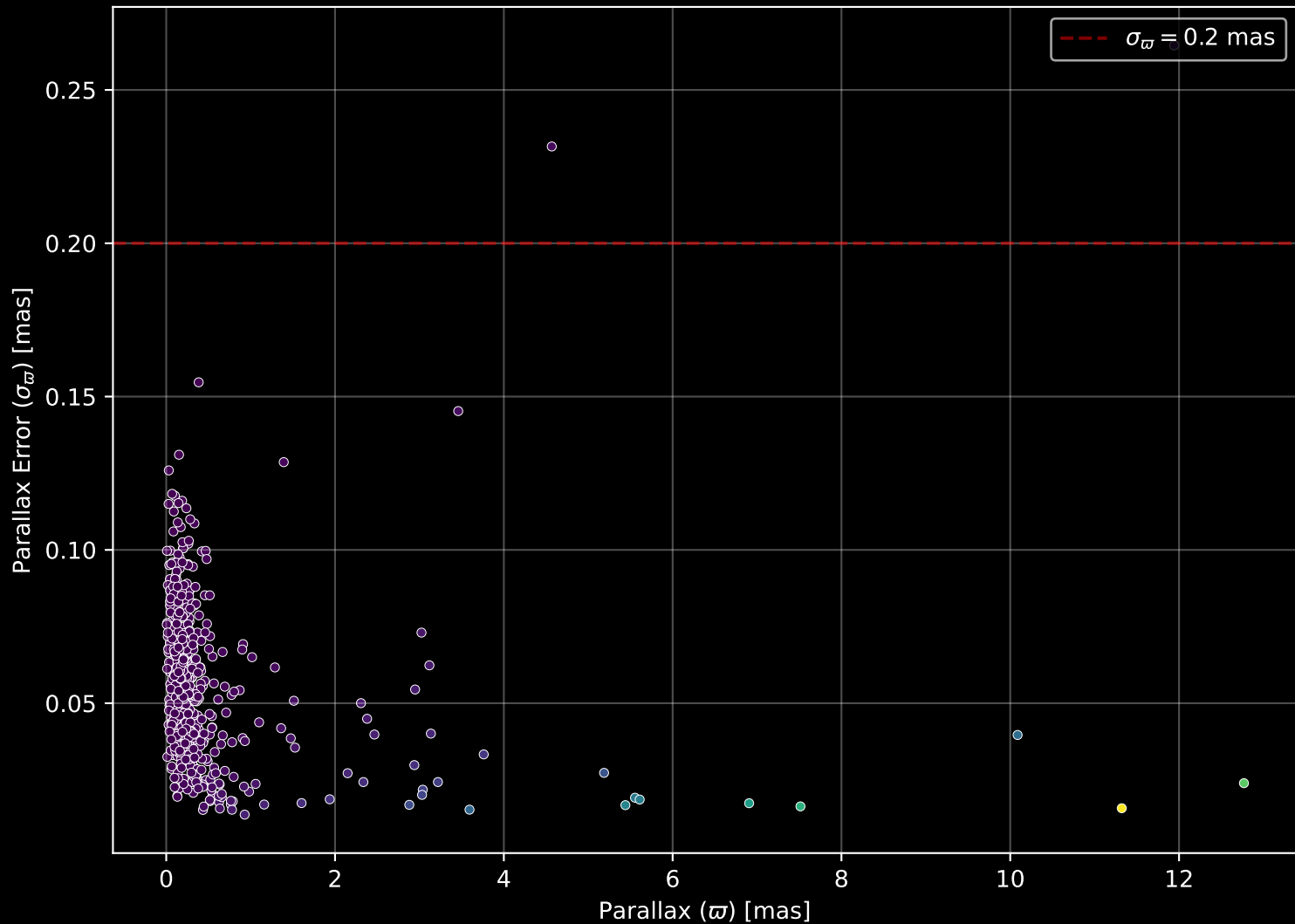
APOGEE DR17 Field: [020+06] Parallax Quality (n= 605)
