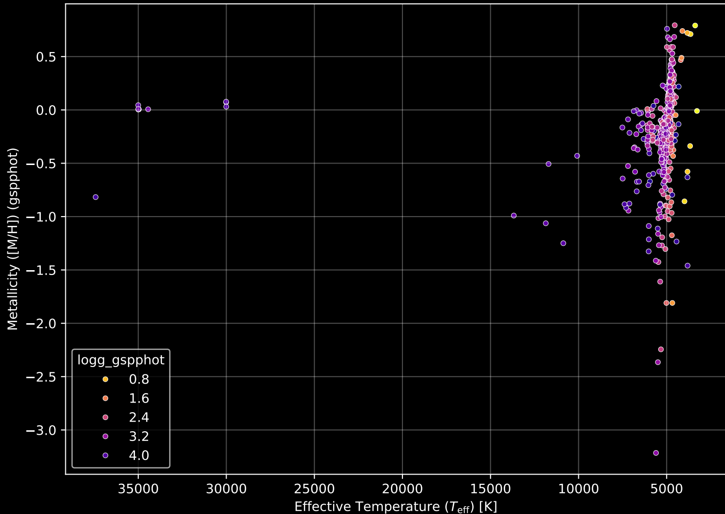
APOGEE DR17 Field: [020+06] Stellar Population Parameters (n= 605)
