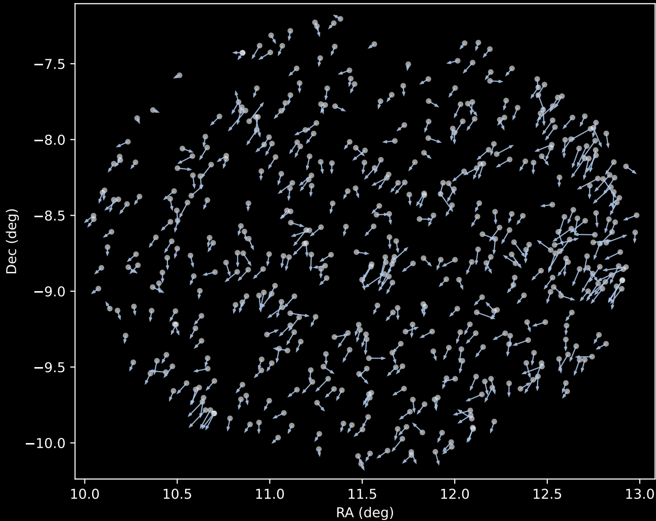
APOGEE DR17 Cluster 1 Proper Motion Vectors (n=509)
