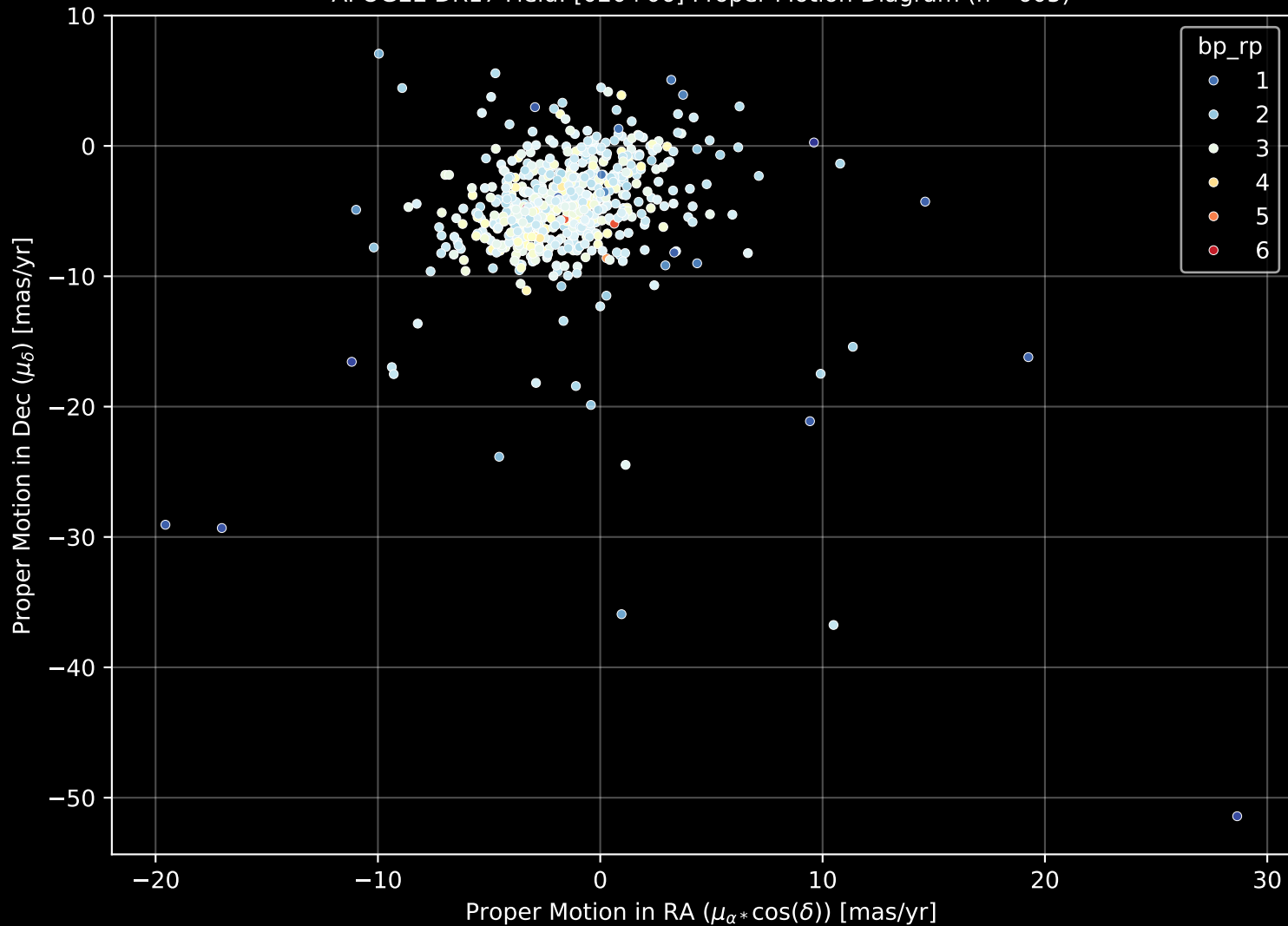
APOGEE DR17 Field: [020+06] Proper Motion Diagram (n= 605)
