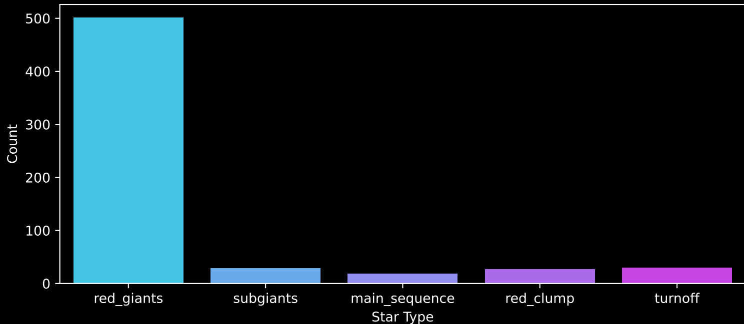
APOGEE DR17 Field: [020+06] Count plot of Star Type
